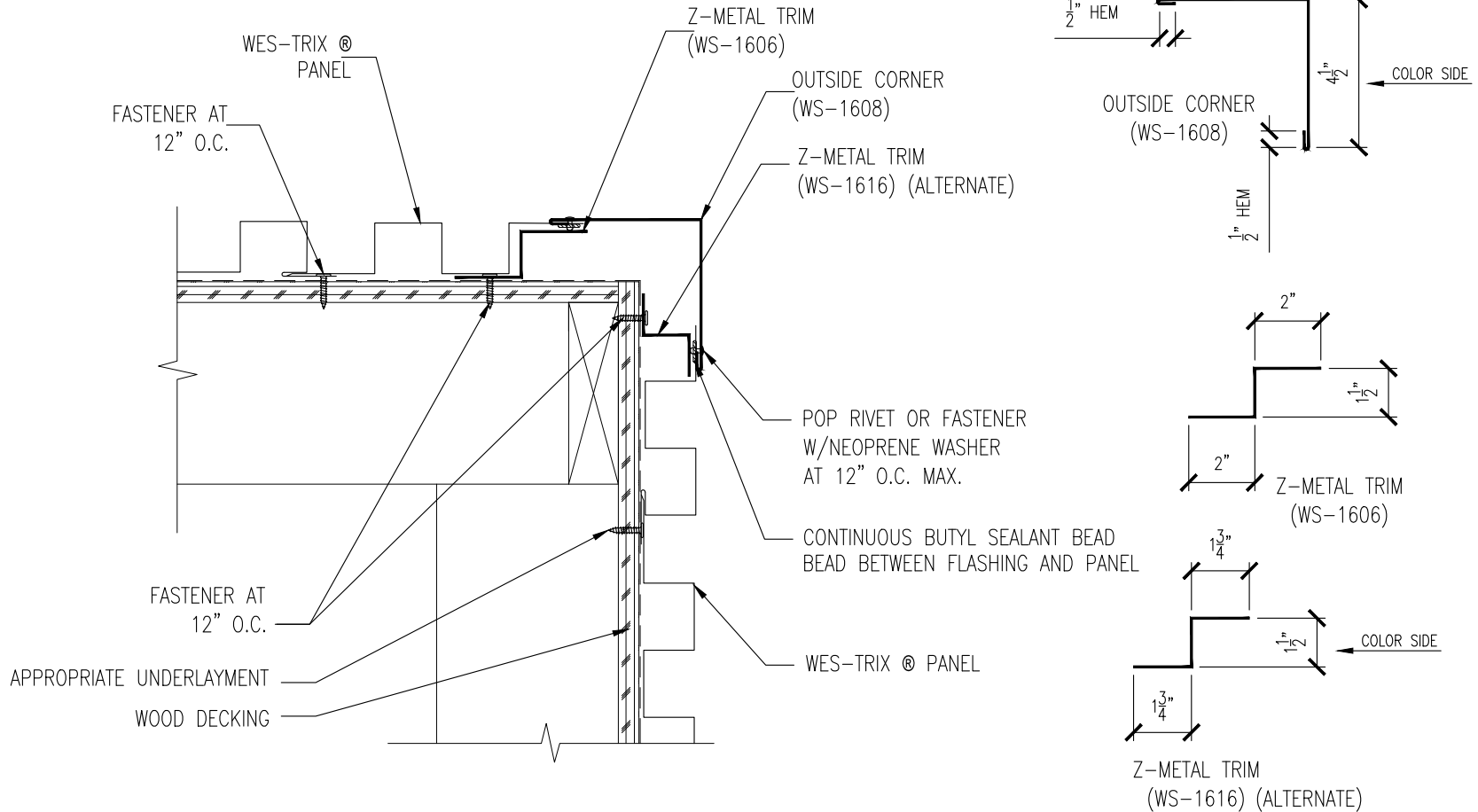
VERTICAL WALL INSTALL
