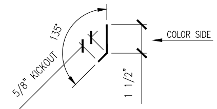
CONTINUOUS CLEAT (WS-1613)
