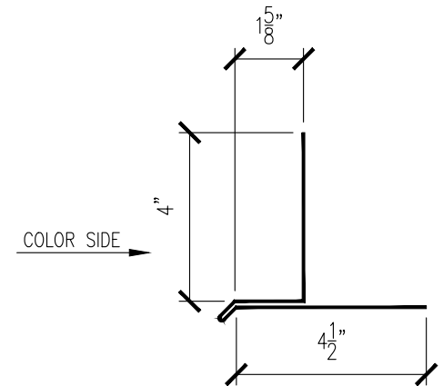
DOOR/WINDOW HEAD TRIM (WS-1610)
