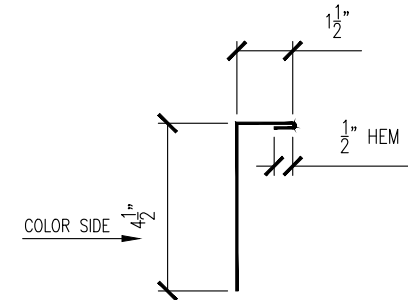
WINDOW/DOOR JAMB TRIM (WS-1611)
