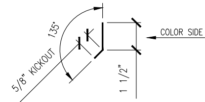
CONTINUOUS CLEAT (WS-1613)
