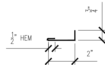
ALTERNATE WALL TRIM (WS-1614)
