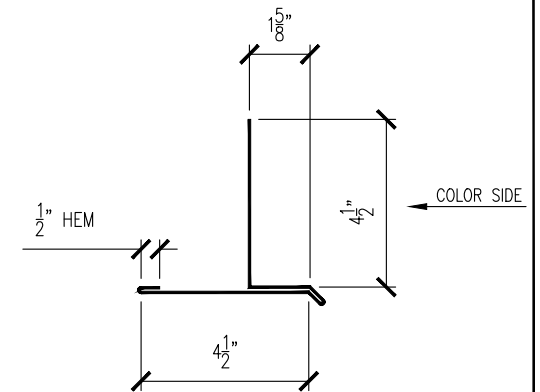
ALTERNATE SILL DRIP TRIM (WS-1605)
